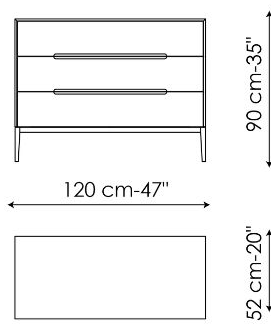
Drawer chest Width: 120cm Depth: 52cm Height: 90cm
