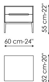
Bedside table low with two drawers Width: 60cm Depth: 52cm Height: 55cm
